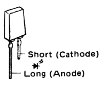
AA-5541K (Orange)
